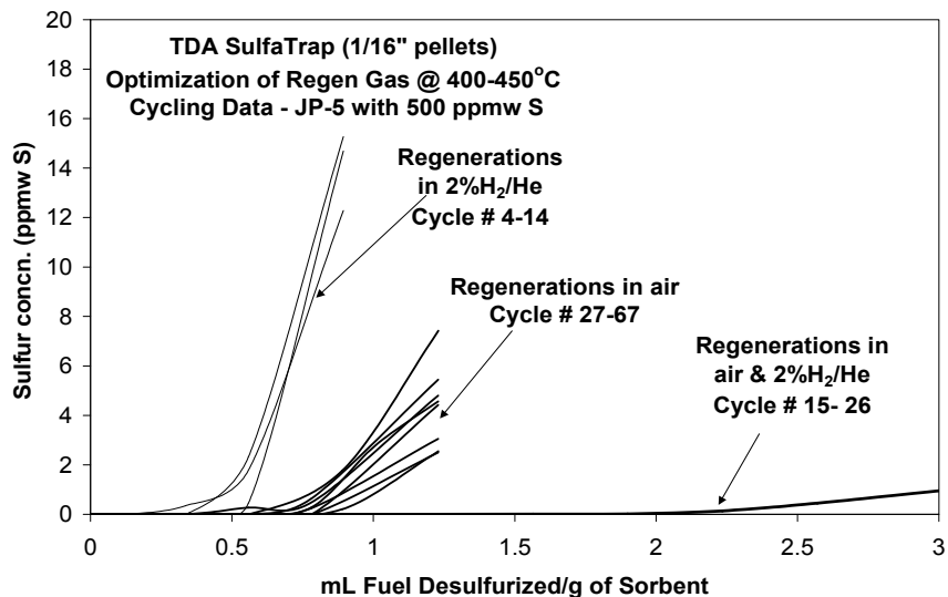
Figure 5. The impact of regeneration gas on desulfurization of jet fuel by SulfaTrap TM -D1. T = 120°C. LHSV = 0.8 h -1 .
