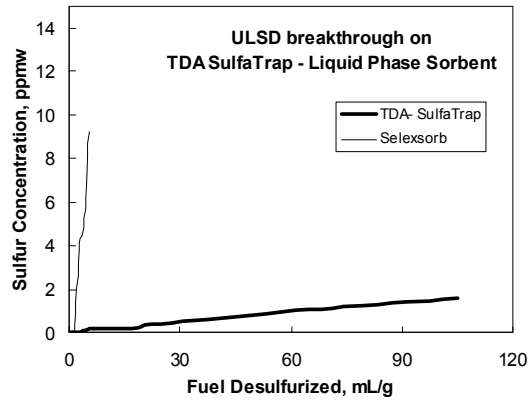
Figure 4. Diesel fuel breakthrough on TDA-SulfaTrap TM -D1 sorbent. T = 120°C. LHSV = 1.6 h -1 .
