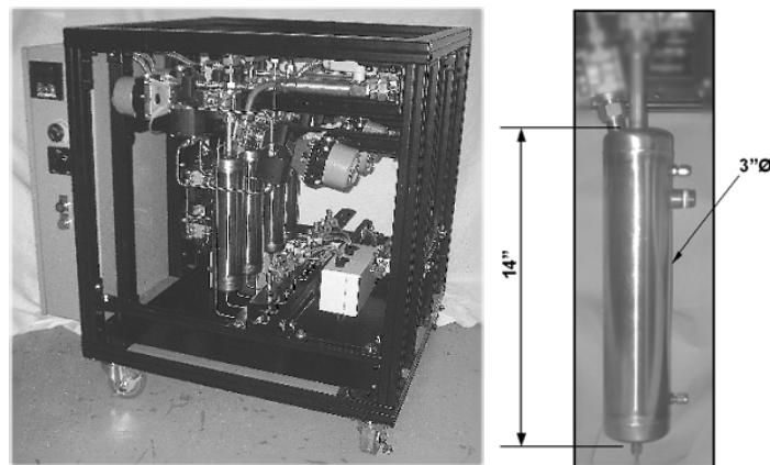
Figure 7. TDA's 4-bed prototype jet fuel desulfurization system.
