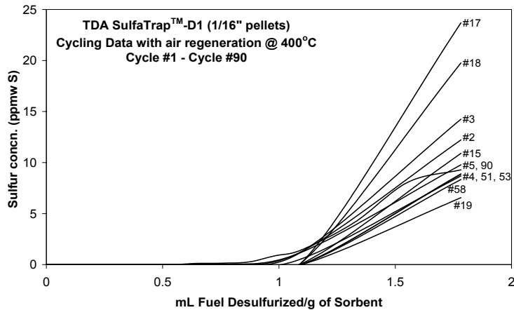
Figure 6. Multiple cycle Test results with JP-5 (500 ppmw S) on TDA-SulfaTrap™-D1 sorbent. T = 120°C. LHSV = 0.8 h -1 .
